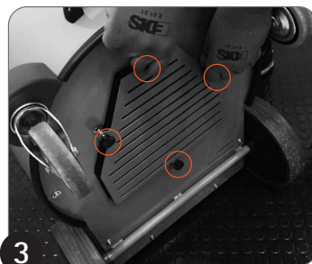
3 Unscrew the 4 knobs
